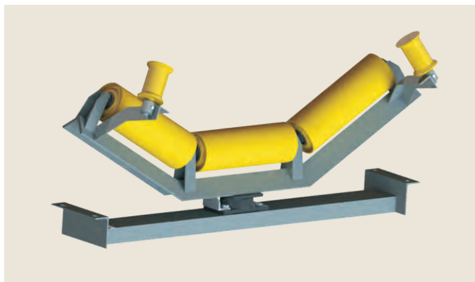
普通槽型调心托辊组 Normal troughing self-aligning idler
