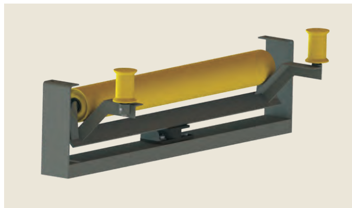
普通平行调心托辊组 Normal flat self-aligning idler
