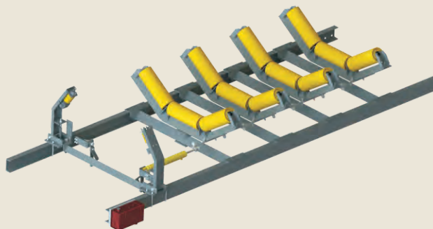
液压调心托辊组 Hydraulic self-aligning idler
